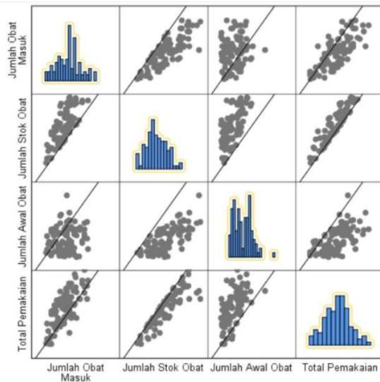
Gambar 1 Scatterplot Matrix
