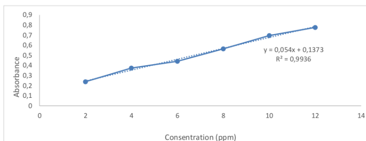
Figure 2. Standard Curve of Vitamin C Solution
