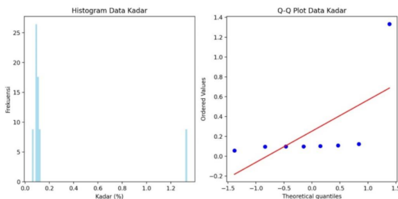
Gambar 1. Histogram dan Q-Q plot uji normalitas Shapiro-Wilk
